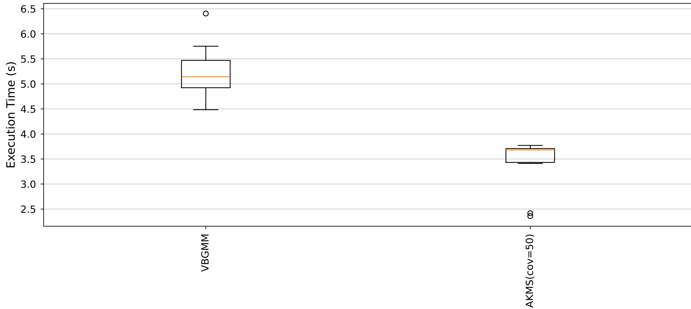
YARA Rules Execution Time Distribution (Cluster3_Size53 dataset)
